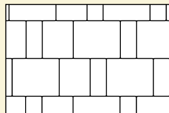
Type 1, 2, 3 Random Runner Bond Pattern Type 1 comprises 50% of total area Type 2 comprises 34% of total area Type 3 comprises 16% of total area
